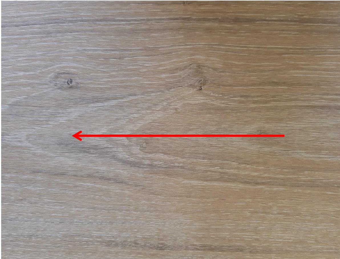
Figure 1: Vinyl Titan Comfort 5mm plank Arrow indicates direction of testing
